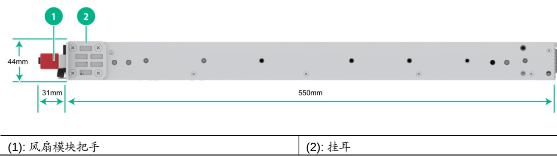
图2-5 S9600XP-24B16DH-G 挂耳安装在电源侧时尺寸示意
