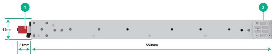
图2-4 S9855-48B 挂耳安装在端口侧时尺寸示意
